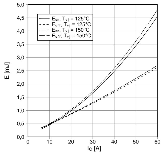
Schaltverluste IGBT-Wechselr. (typisch) switching losses IGBT-inverter (typical) E_{on} = f(I_C) , E_{off} = f(I_C) V_{GE} = \pm 15\text{ V} , R_{Gon} = 56\ \Omega , R_{Goff} = 56\ \Omega , V_{CE} = 300\text{ V}
